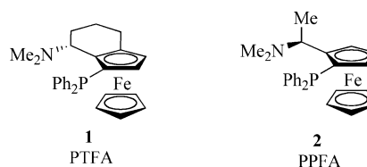
Figure 1. The PTFA and PPFA ligands.
