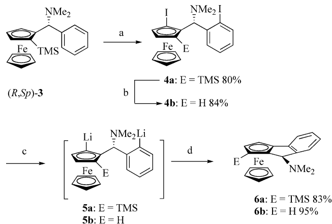
Scheme 1. Reagents and conditions: (a) t BuLi (2.4 equiv.) in diethyl ether, 0 °C, 2 h, then I 2 (2.5 equiv.) in DMSO, room temp., 15 h; (c) n BuLi (2.5 equiv.) in diethyl ether, 0 °C, 2 h; (d) Fe(acac) 3 (3.0 equiv.), 0 °C 10 min, then room temp., 22 h.
