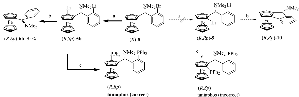
Scheme 3. Reagents and conditions: (a) t BuLi (3 equiv.) in diethyl ether, 0 °C, 2 h; (b) Fe(acac) 3 (3 equiv.), 0 °C 10 min, then room temp., 22 h; (c) Ph 2 PCl (2.5 equiv.), –78 °C, 1 h.
