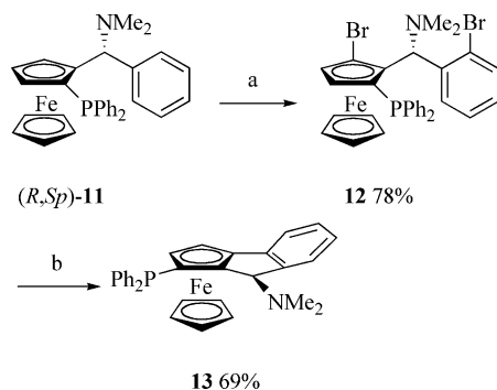
Scheme 4. Reagents and conditions: (a) t BuLi (2.5 equiv.) in diethyl ether, 0 °C, 2 h, then BrCF 2 CF 2 Br (3.0 equiv.); (b) t BuLi (2.5 equiv.) in diethyl ether, 0 °C, 2 h, then Fe(acac) 3 (3.0 equiv.), 0 °C 10 min, then room temp., 22 h.
