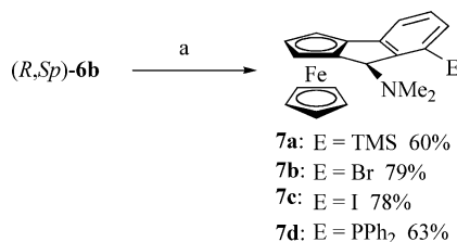
Scheme 2. Reagents and conditions: (a) t BuLi (1.3 equiv.) in diethyl ether, 0 °C, 2 h, then E + (1.0 equiv.).
