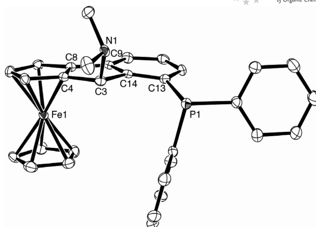
Figure 2. X-ray structure of 7d . Selected bond lengths [Å]: C3–C4 1.511, C3–C14 1.537, C4–C8 1.428, C8–C9 1.473, C9–C14 1.411, C13–C14 1.388, N1–C3 1.524, P1–C13 1.842. Selected bond angles [°]: C3–C4–C8 110.3, C4–C3–C14 101.8, C8–C9–C14 107.8, C3–C14–C9 111.0, C9–C14–C13 121.7, C3–C14–C13 127.0, P1–C13–C14 116.14, N1–C3–C4 111.7, N1–C3–C14 111.5.
